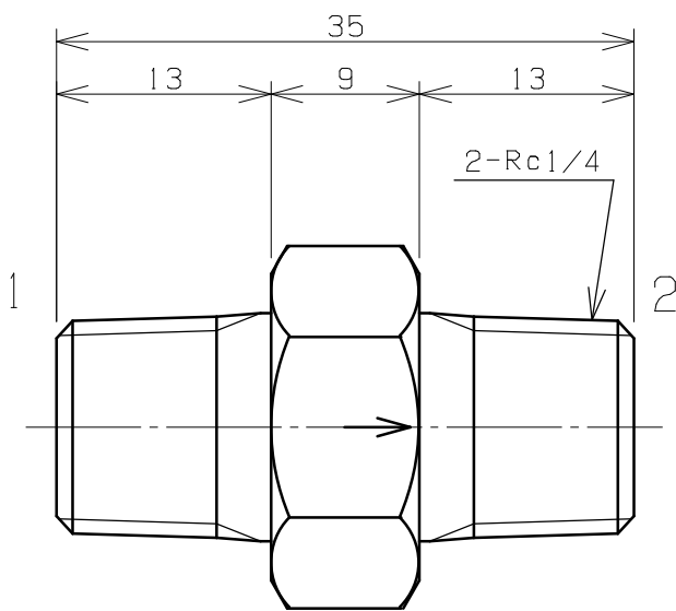
Male Nipple Check Valve Model 0289B
